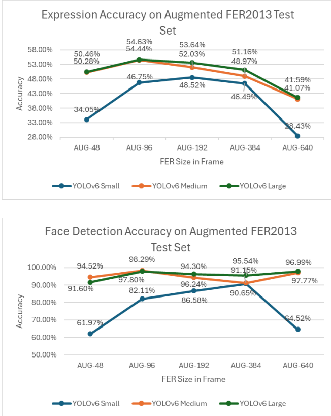
Figure 3. Our model's classification (top) and face detection (bottom) accuracy on augmented FER2013 test set with various
