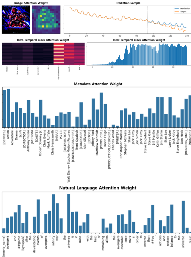
(Figure 4) Visualization of Sample Attention Weights
