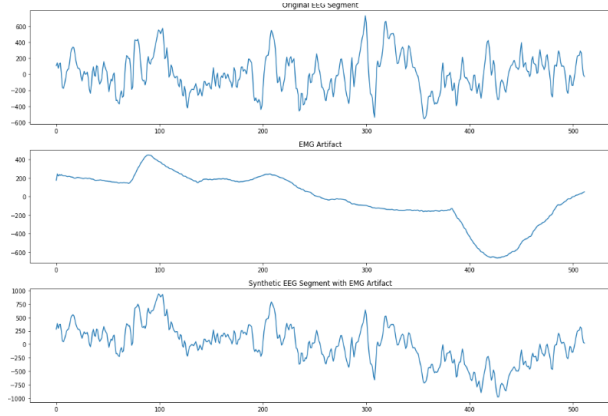
Fig. 1. Example of contaminated signal using Linear Mixing method
