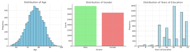
Fig. 2. Visualization of Demographic Information
