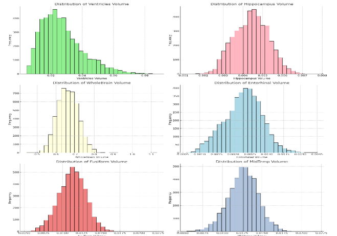
Fig. 4. Visualization of Brain Measurements (biomarkers)
