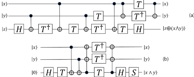
<그림 4> (a)Standard decomposition of Toffoli-gate used in Qiskit (b)Gidney's relative-phase (GRT) Toffoli-gate decomposition
