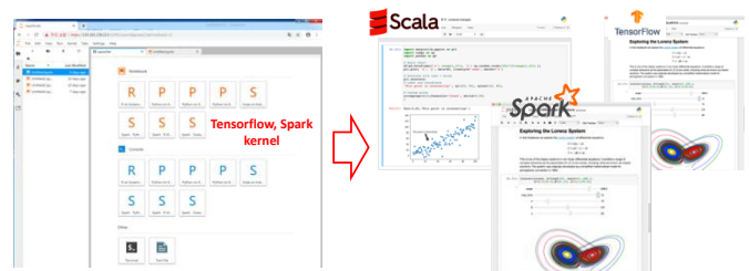
Fig. 3. Jupyter Service.
