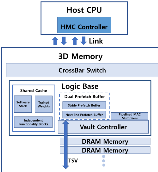
(그림 1) Overall Architecture
