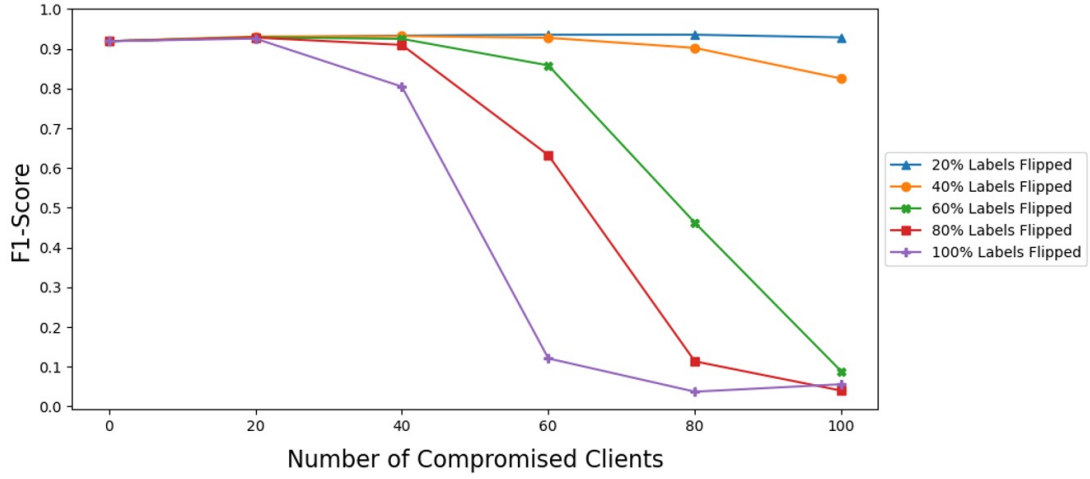
Figure 4: F1-Score vs Compromised Clients and Flipped Labels for Car-Hacking
