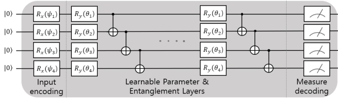
Fig. 1. Illustration of QNN with the input |\psi\rangle , the parameter \theta and linear entanglement structure.
