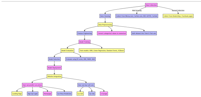
Fig. 2. System Architecture.
