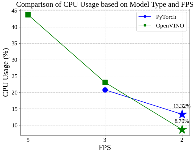
Fig. 3: Impact of FPS adjustments and hardware-specific optimizations on CPU utilization in the YOLOv8 Nano within the RGB-D package. The camera node is also active when the "\rgb_d_detection" node in Fig. 2a is active.
