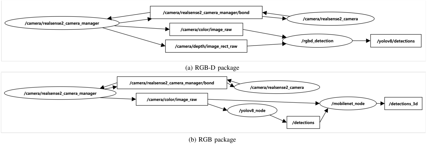
Fig. 2: Comparison of RQT graphs between RGB-D and RGB packages.
