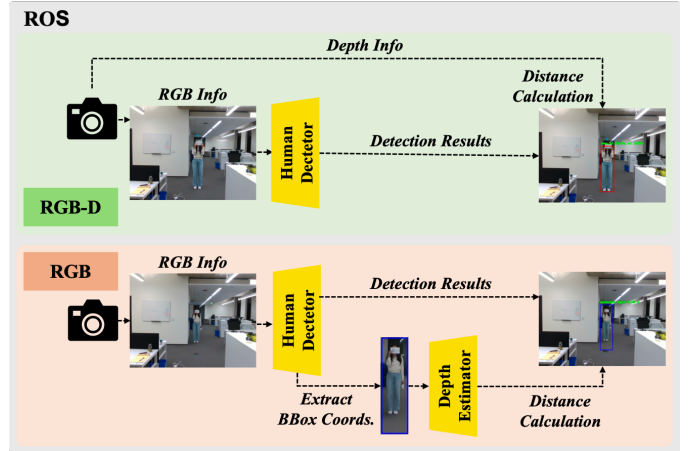
Fig. 1: The overall pipeline of our ROS packages. Within the RGB-D package, the camera furnishes both depth data and RGB information from real-time streaming video. In contrast, the RGB package provides solely RGB data, necessitating the extraction of depth information through a depth estimator. Ultimately, both packages visualize the estimated distance and bounding box coordinates superimposed on the real-time data stream.
